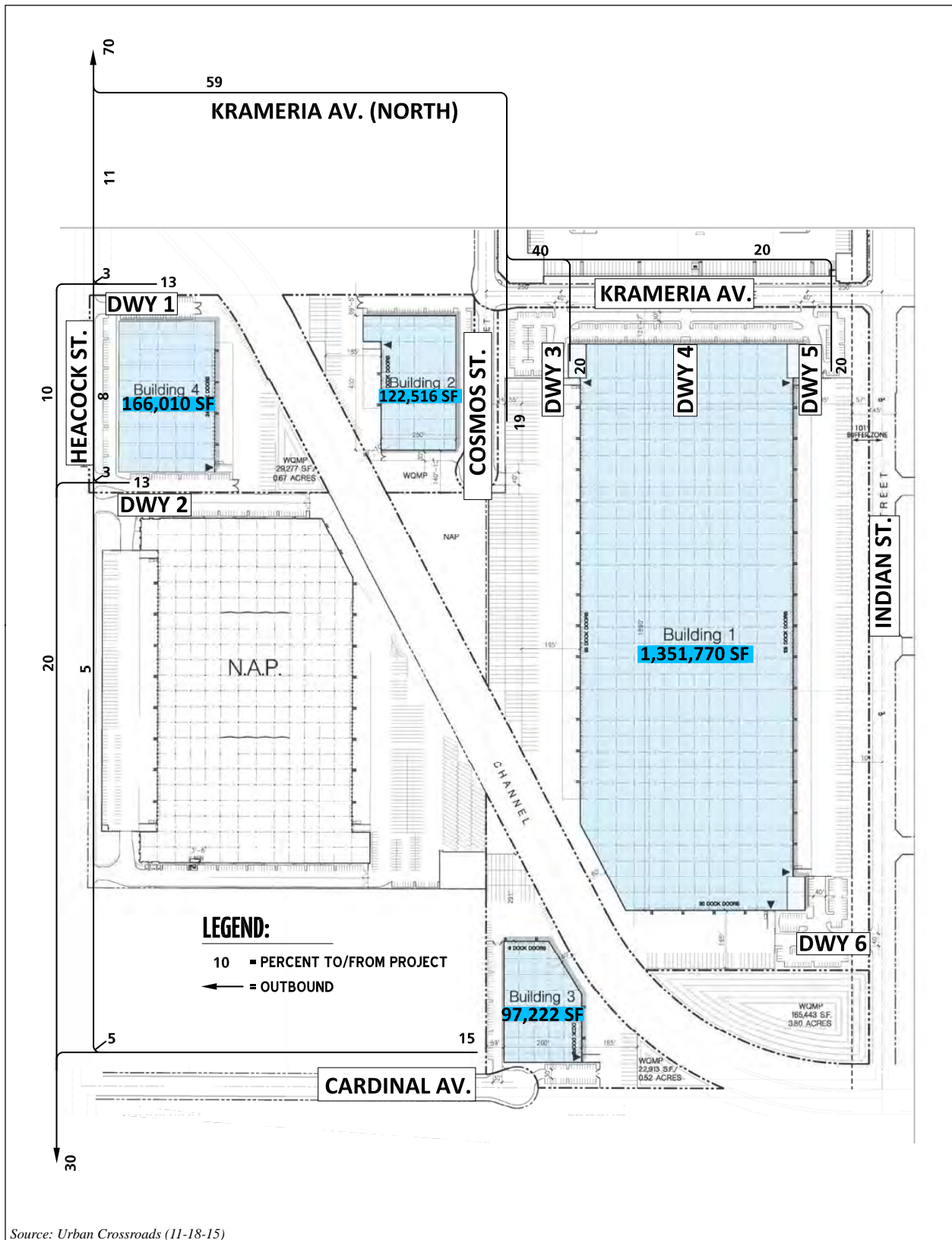
Figure 4.11-10 PROJECT TRUCK TRIP DISTRIBUTION (WITHOUT INDIAN STREET BRIDGE) (2 OF 2)
