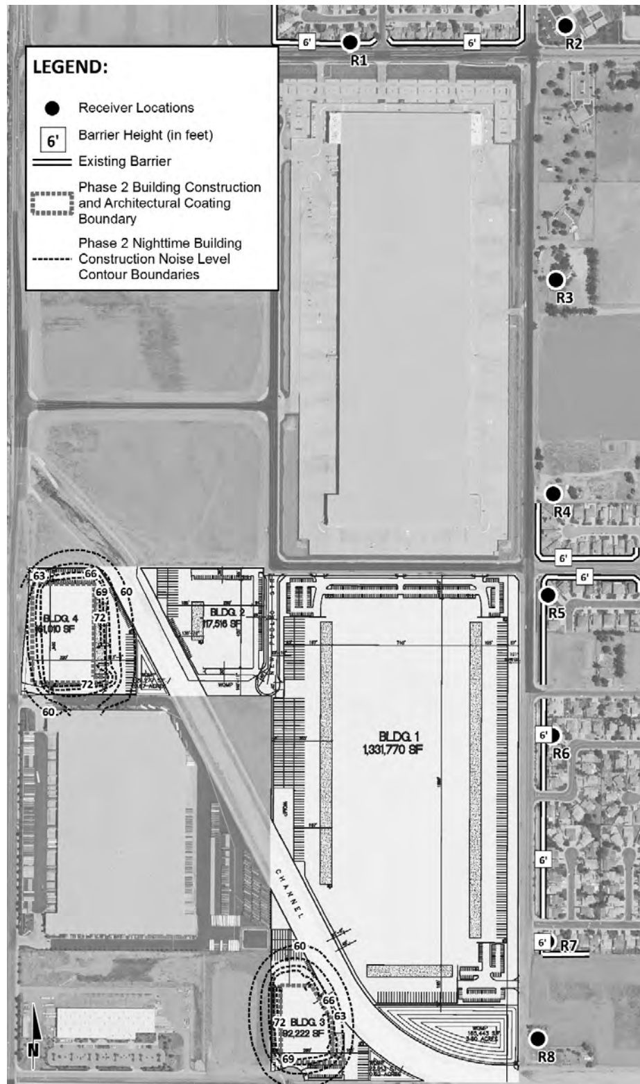
Figure 4.10-11 PHASE 2 NIGHTTIME BUILDING CONSTRUCTION EQUIPMENT NOISE CONTOURS
