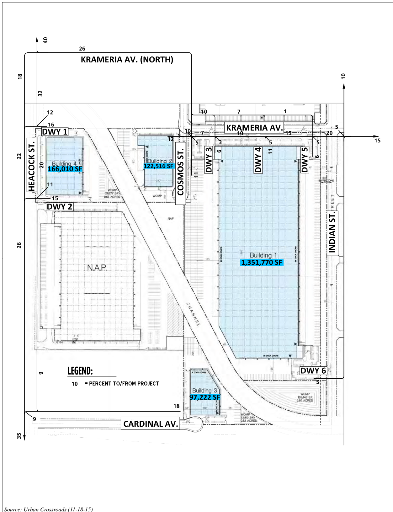
Figure 4.11-9 PROJECT PASSENGER CAR TRIP DISTRIBUTION (WITHOUT INDIAN STREET BRIDGE) (2 OF 2)
